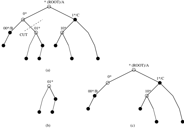
Fig. 4. Cutting a trie: (a) Original trie (b) Child sub-trie (c) Parent trie. Dark circles are used to indicate prefix nodes, while the light circles represent non-prefix (zero weight) nodes required for building the trie.
