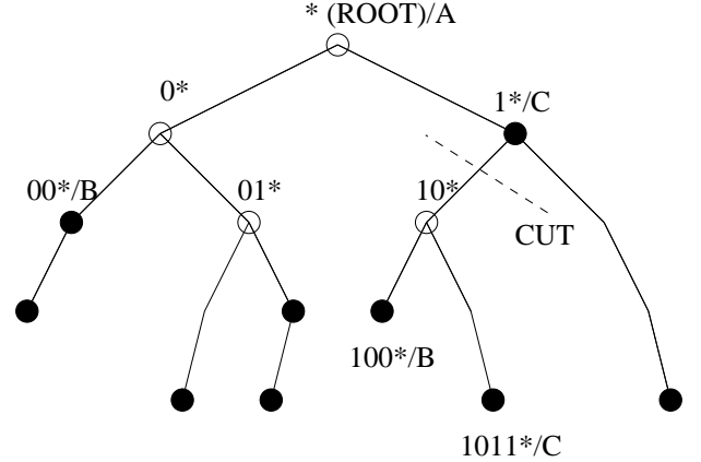
Fig. 5. Before partitioning, the string 10101100 will match the prefix 1* and the lookup will take three memory accesses (root-1*-10*). After partitioning, the lookup starts directly at the root of the child sub-trie (10*), and ends after one memory access. Thus the loads of parent and child tries after partitioning should be 0 and 1 respectively. However, simply adding the weights of nodes in each partition would give the loads of parent and child as 2 and 0 respectively.
