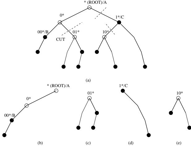
Fig. 7. (a) Original trie. (b), (c), (d), and (e) are partitions formed after cutting (a).
