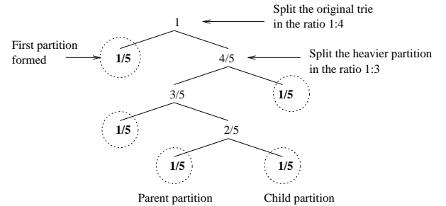
Fig. 6. The figure shown an example of creating 5 partitions. Note that the tree depicts the flow of the partitioning algorithm; it is not a trie. Each level of the tree structure represents a single iteration of partitioning. The root node indicates the load of the original trie normalized to 1. Each number in the tree represents the load of a trie relative to the load of the original trie. The left and right branches indicate the loads of the parent and child tries obtained by cutting a trie. Numbers in boldface represent the load of the final partitions.
