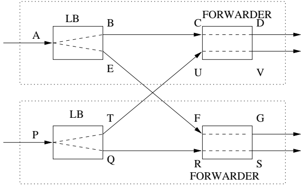
Fig. 8. LB: Load Balancer. The figure depicts two processing elements (dotted boxes) of a distributed router working in parallel. Each processing element stores only a part of the entire forwarding table, as determined by the partitioning algorithm.
