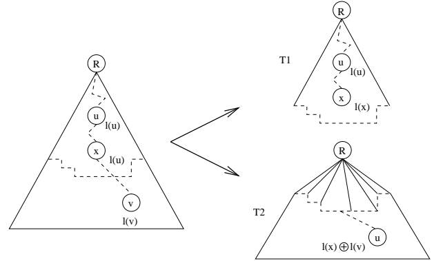
Fig. 3. Splitting the trie [29].
